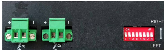
DIP-switch Bank Locations
