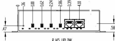
RJ45 UPLINK CONFIGURATION
