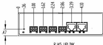
RJ45 UPLINK CONFIGURATION
