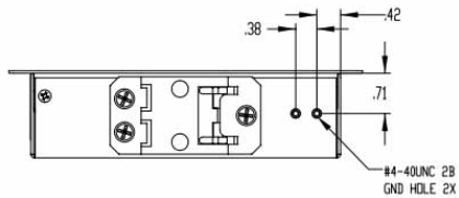
SFP UPLINK CONFIGURATION
