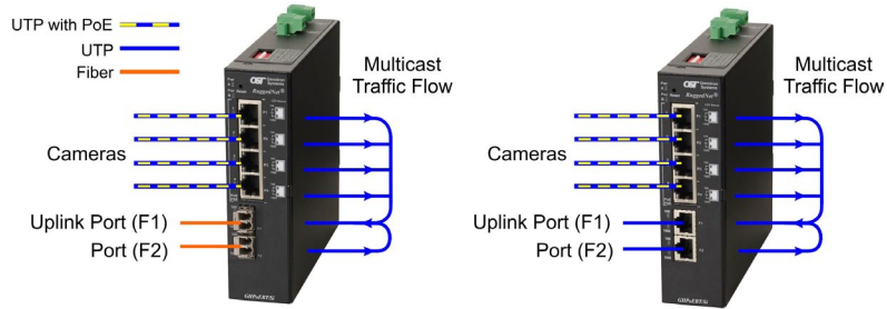
Directed Switch Mode Dual Uplink Port
