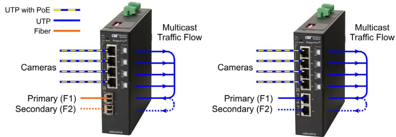
Directed Switch Mode with Uplink Redundancy
