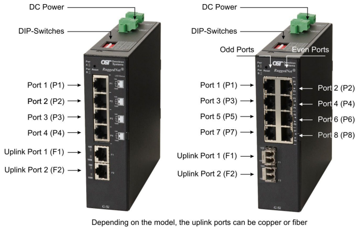
Front Panel Layout
