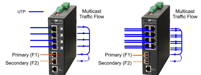
Directed Switch Mode with Uplink Redundancy
