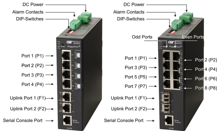
Front Panel Layout
