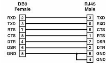
Standard RJ-45 to DB-9 serial cable pin-out
