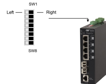
DIP-switch Bank Locations
