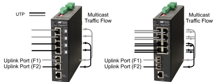
Dual Device with Directed Switch Mode
