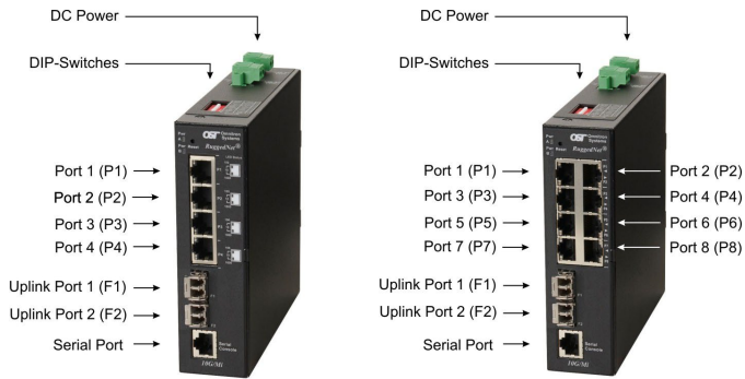
Front Panel Layout
