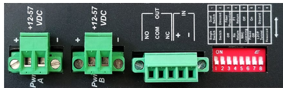
Top View - Location of DC Power, Alarm Contacts and DIP-switches
