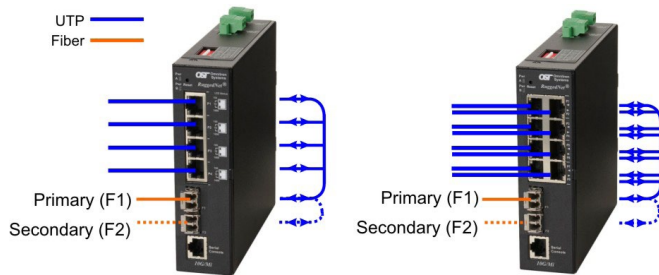
Redundant Uplink
