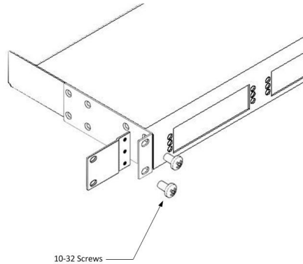
Bracket Installation
