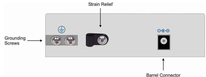
AC Models Rear View: Barrel Connector for AC/DC Power Adapter
