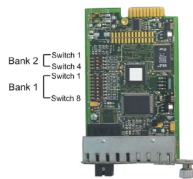
DIP-switch Location
