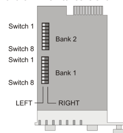
DIP-switch Location
