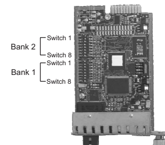
Figure A: DIP-Switch Locations
