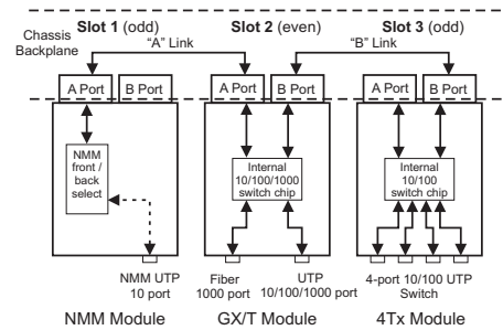
Fig. 1 In-Band Managed GX/T Application
