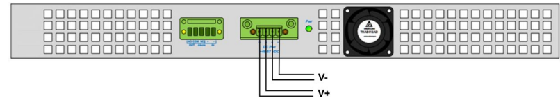
DC Models Rear View: Power Connections
