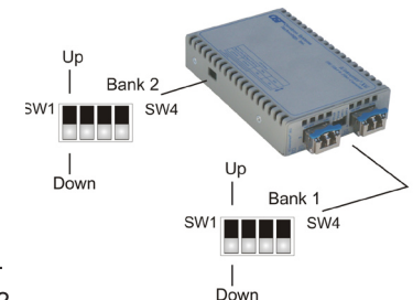
Figure 1: DIP-switch Location
