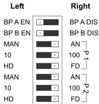
4 Port Switch Module Default DIP-Switch Settings
